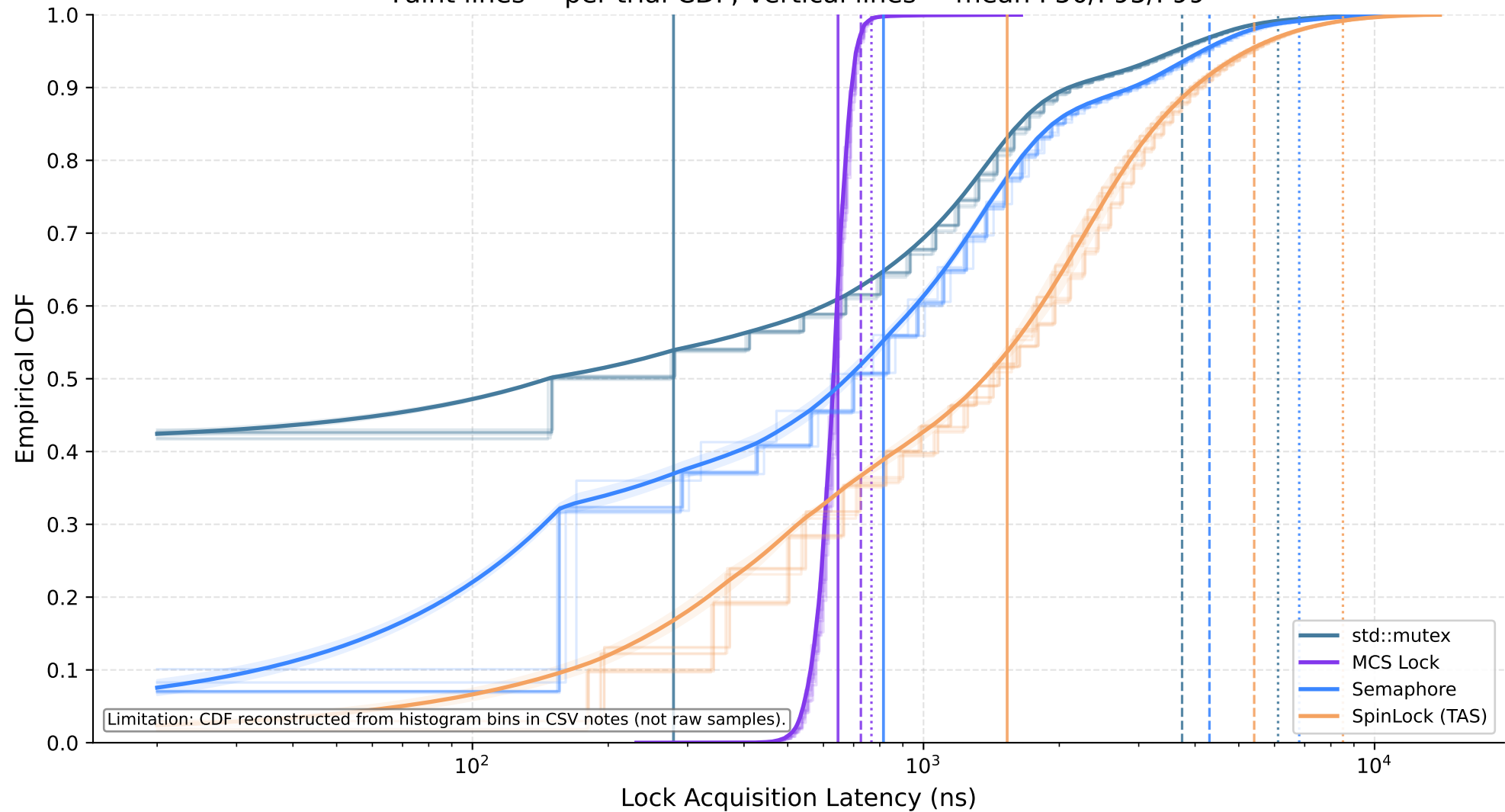
Fig 10 — Empirical CDF from Histogram Bins (threads=8) Faint lines = per-trial CDF; vertical lines = mean P50/P95/P99
